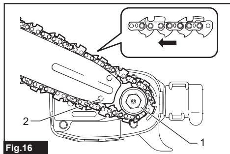
Fig.16 1. Pignon 2. Orifice
